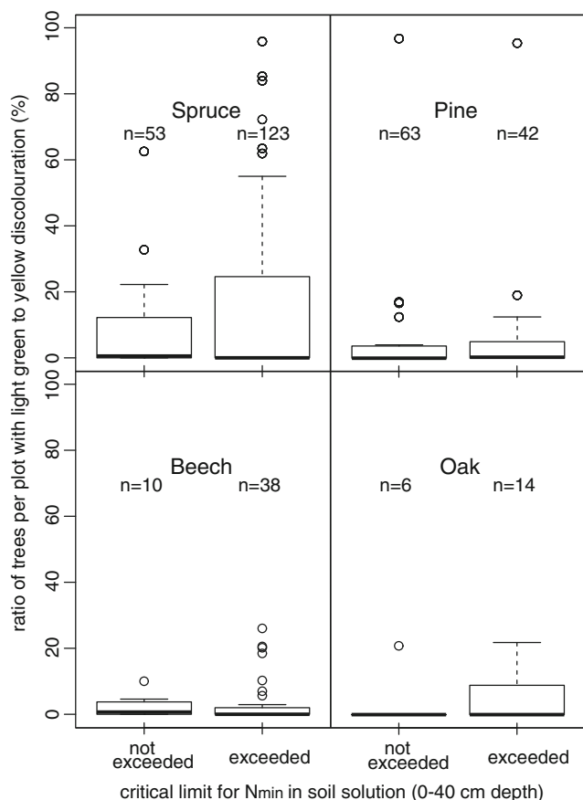
Fig. 2 Percentage of trees per plot ( f_y > 50\% ) with reported foliage discolouration ( light green to yellow ) for the species groups spruce, pine, beech and oak for plots with and without exceedance of the critical limits for inorganic N in soil solution ( N_{min} < 1 ) in the majority of samples ( f_{ss} > 50\% ) from the depth of the deepest lysimeters per plot
