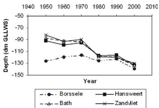
Figure 5. Channel depth at 4 locations in the Westerschelde (GLLWS ¼ level at averaged minimal low spring tide) (based on data of the Ministry of Transport, Public Works and Water Management of the Netherlands).
