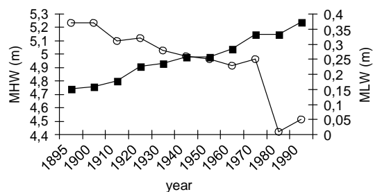
Figure 7. Evolution of mean high water level (MHW, squares) and mean low water level (MLW, open circles) in the Scheldt estuary near Antwerpen (based on data of the Maritime Access Division of the Flemish Government).
