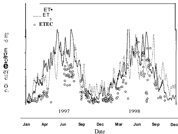
Fig. 8. Daily totals of the evapotranspiration (lower panel), measured by the eddy covariance technique (ETEC; open circles) on dry days, and seven day running means of evapotranspiration as simulated by the models WAVE (ETw; solid line) and SECRETS (ETs; dashed line) in a 70-year-old Scots pine ( Pinus sylvestris L.) stand in the Campine region, Northern Belgium for 2 consecutive years (1997, 1998).
