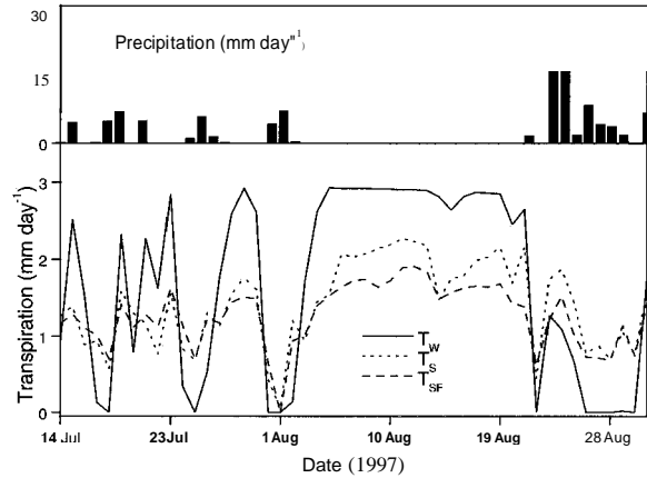
Fig. 4. Precipitation (upper panel) and daily totals of transpiration (lower panel) of a 70-year-old Scots pine ( Pinus sylvestris L) stand in the Campine region, Northern Belgium during the sap flow measurement campaign of 14 July to 31 August 1997. Transpiration estimates by the sap flow method ( T_{sF} ; dashed line), the WAVE model ( T_w ; solid line), and the SECRETS model ( T_s ; pointed line) are being presented.
