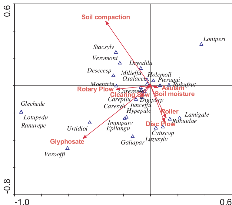
Figure 2. Species ordination diagram based on Canonical Correspondence Analysis, with respect to two quantitative variables (soil compaction and moisture) and eight nominal variables (asulam, glyphosate, brush cutter, clearing saw, disc plow, roller, rotary plow, harrow). For legibility reasons, only the species having the best fit are represented. The axes (1: horizontal; 2: vertical) are scaled in standard deviation units. Eigenvalues of first and second axis were: site 0.087 and 0.052, respectively. Species abbreviations are based on the first four letters of genus and species names (for full names, see Fig. 1).
