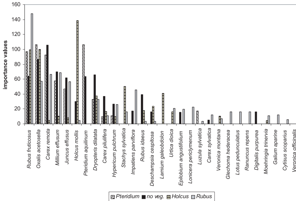
Figure 1. Herbaceous species which developed four years after treatments in the experimental areas (main feature of understory before treatment is given in the graph legend). Data are importance values based on sum of relative cover and relative frequency. Species are ranked according to their decreasing mean importance value.
